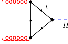
Figure 35: Higgs production in gluon fusion at leading order.
