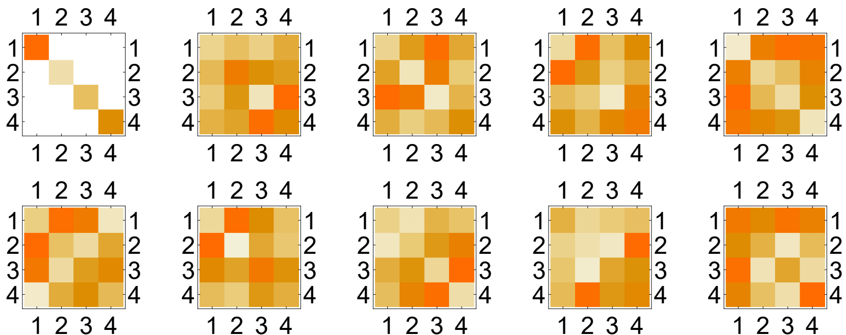
Figure 8: (D, N) = (10, 4) approximate solution \text{Abs} \left[ \widehat{a}_{\kappa\text{-approx-sol-HERM}}^{\prime\mu} \right] with f_{\text{penalty}} = 108.094 . Shown are \mu = 1, \dots, 5 on the top row and \mu = 6, \dots, 10 on the bottom row. (v2: update October 7, 2021)
