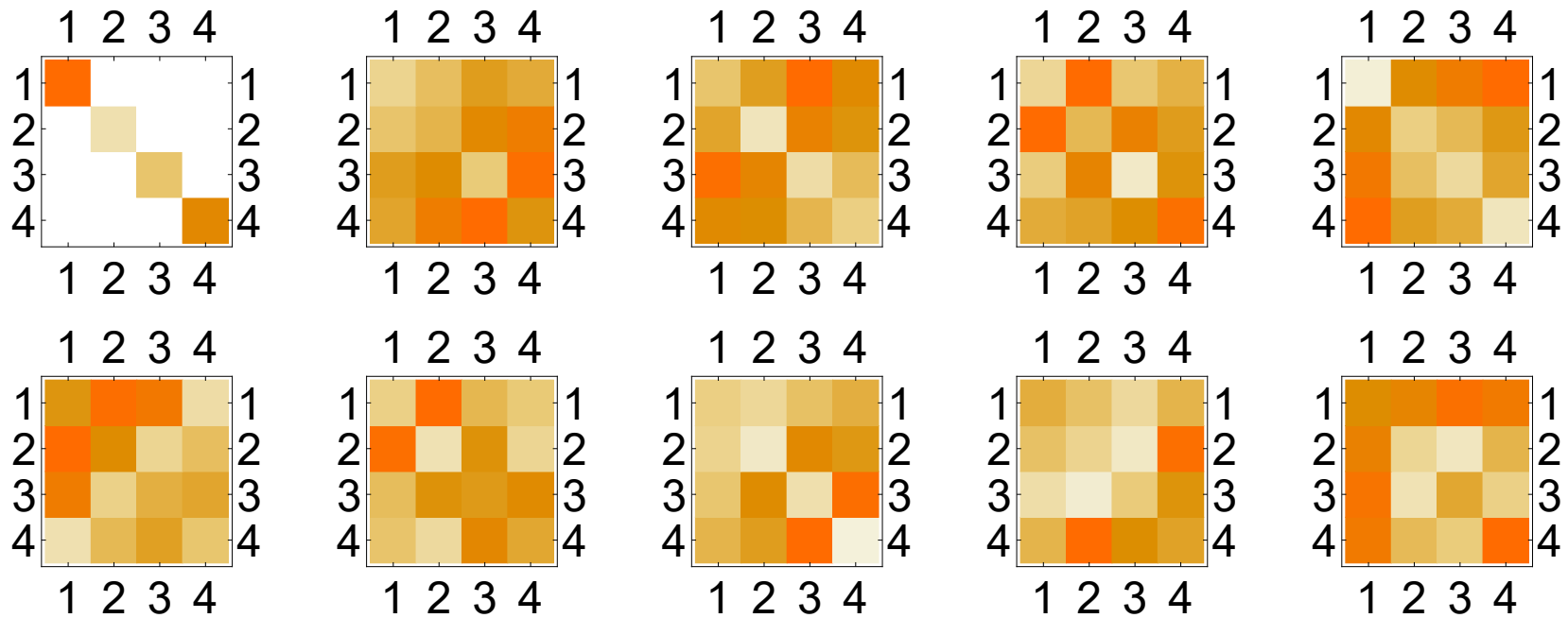
Figure 6: (D, N) = (10, 4) approximate solution \text{Abs} \left[ \widehat{a}_{\kappa\text{-approx-sol-HERM}}^{\prime\mu} \right] with f_{\text{penalty}} = 310.932 . Shown are \mu = 1, \dots, 5 on the top row and \mu = 6, \dots, 10 on the bottom row.
