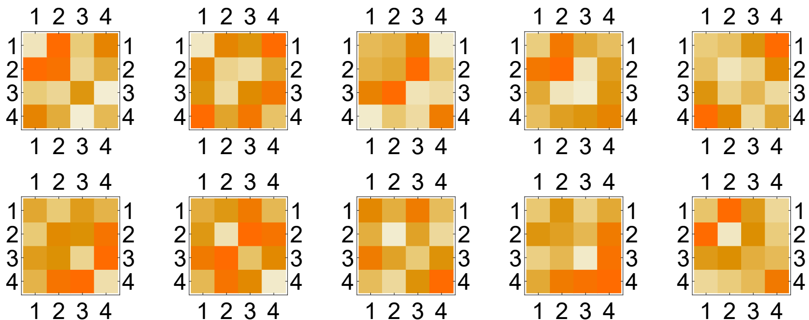
Figure 4: (D, N) = (10, 4) approximate solution \text{Abs} \left[ \widehat{a}_{\kappa\text{-approx-sol-HERM}}^{\mu} \right] with f_{\text{penalty}} = 108.094 . Shown are \mu = 1, \dots, 5 on the top row and \mu = 6, \dots, 10 on the bottom row. (v2: update October 7, 2021)
