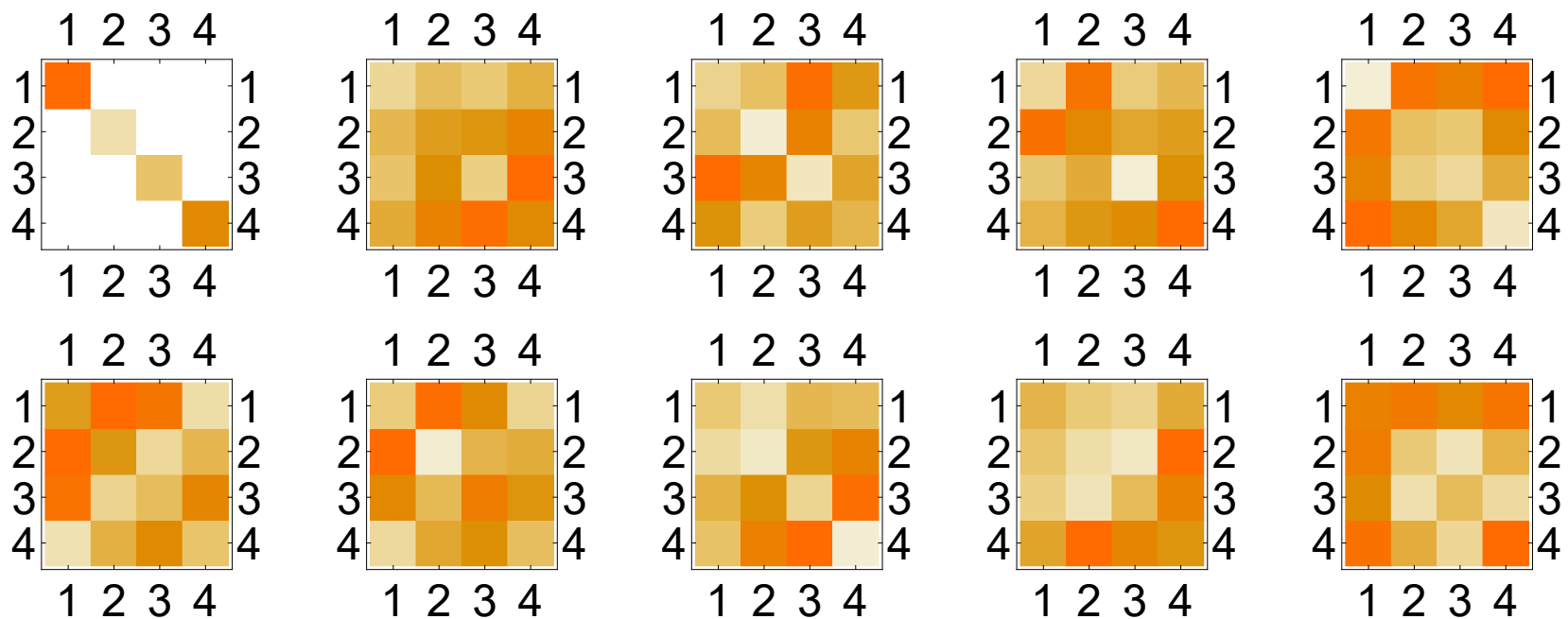
Figure 7: (D, N) = (10, 4) approximate solution \text{Abs} \left[ \widehat{a}_{\kappa\text{-approx-sol-HERM}}^{\prime\mu} \right] with f_{\text{penalty}} = 209.33 . Shown are \mu = 1, \dots, 5 on the top row and \mu = 6, \dots, 10 on the bottom row.
