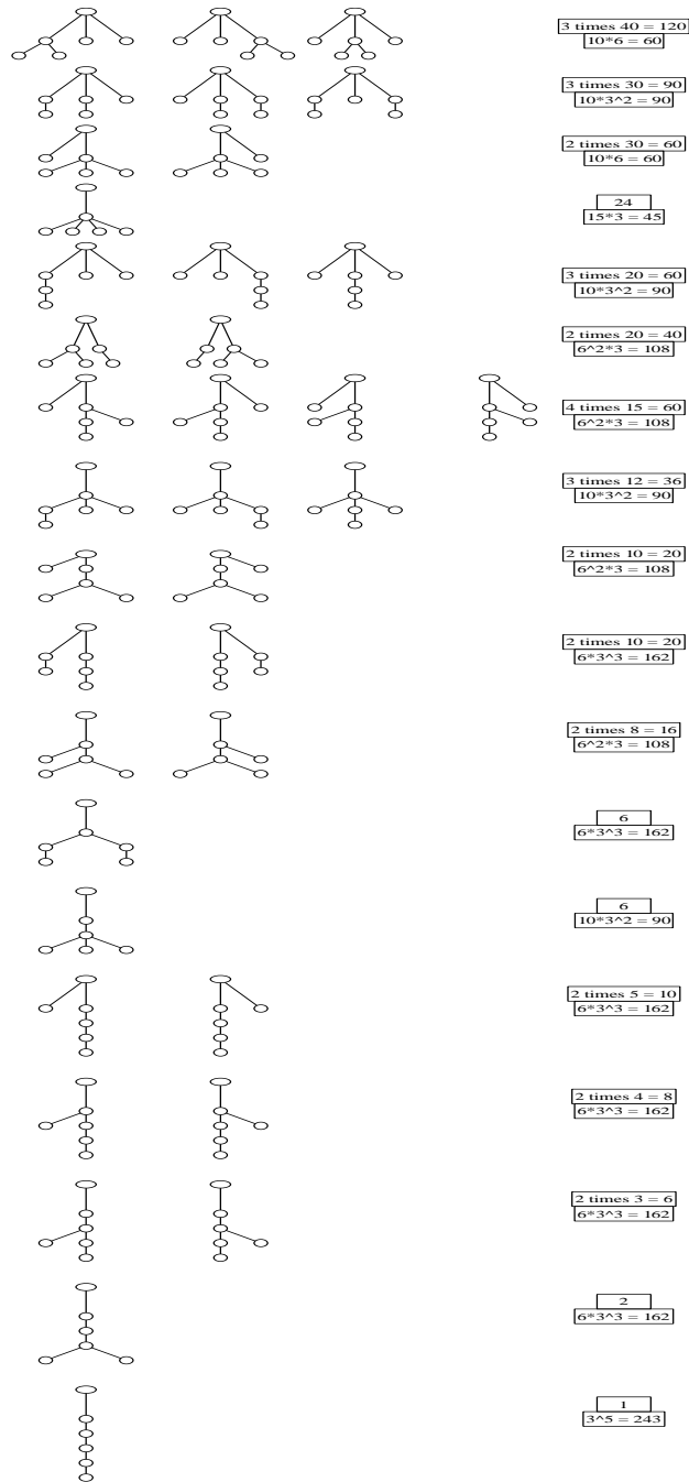
Figure 4: Rooted ordered trees with n = 6 vertices.
